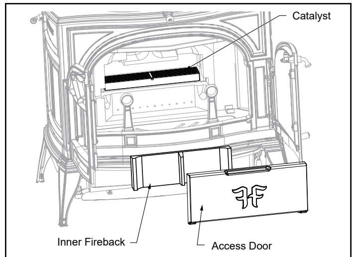
Figure 3.7 - Inspect the catalytic combustor.
