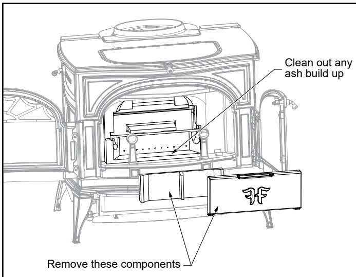
Figure 3.6 - Inspect and clean out ash accumulation behind the combustion system.
