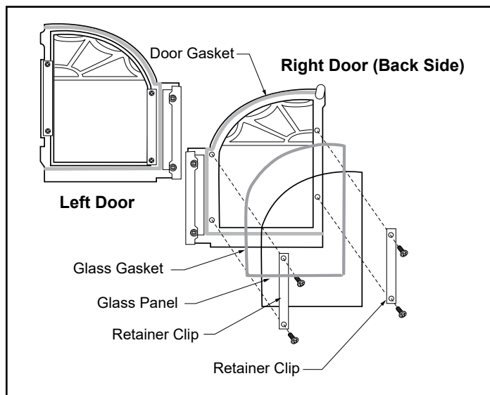
Figure 3.1 - Exploded view of the glass assembly for the right door.
