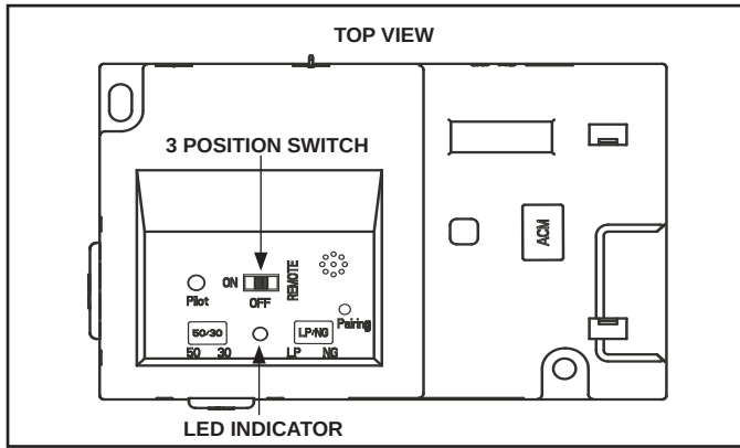
Figure 11.28 IFT-ECM
