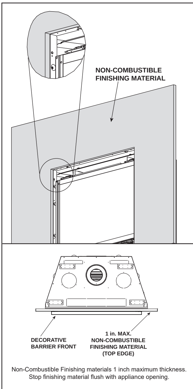
Figure 10.13 Non-Combustible Finishing Material 1 Inch Thick or Less - Overlap Fit Fronts
