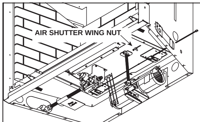
Figure 9.2 Air Shutter
