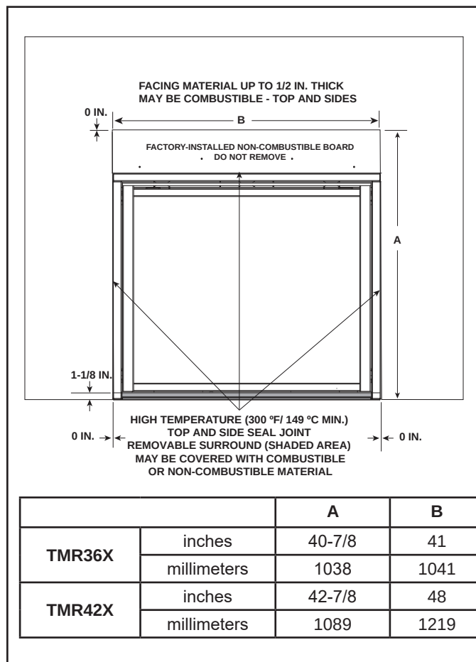
Figure 10.2 Non-combustible Facing Diagram
