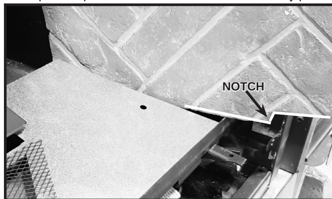
Figure 11.2 Side Refractory Panel Notch
