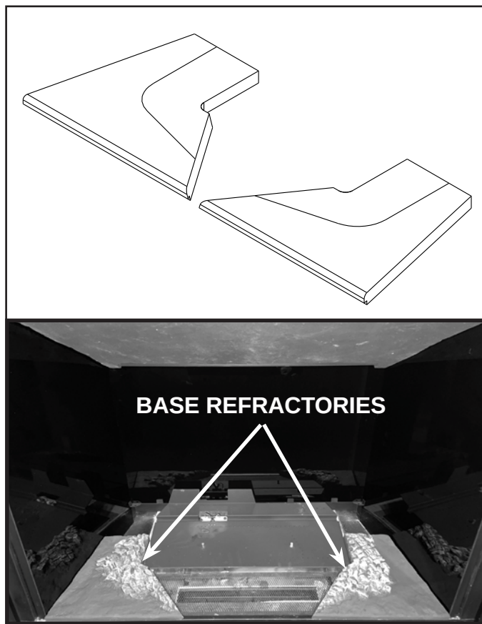
Figure 11.23 Base Refractory Installed
