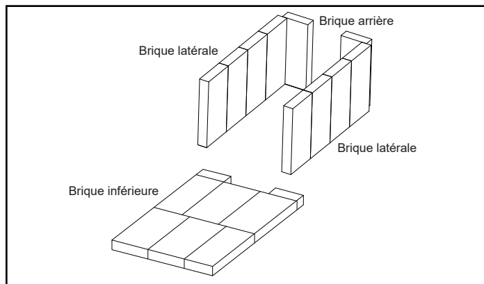
Figure 5.2 - Installer Firebrick
