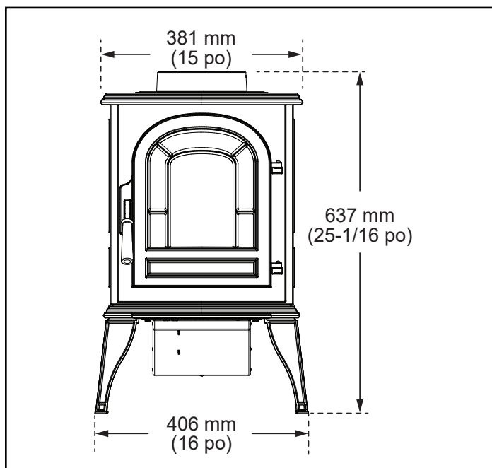
Figure 3.1 – Vue frontale
