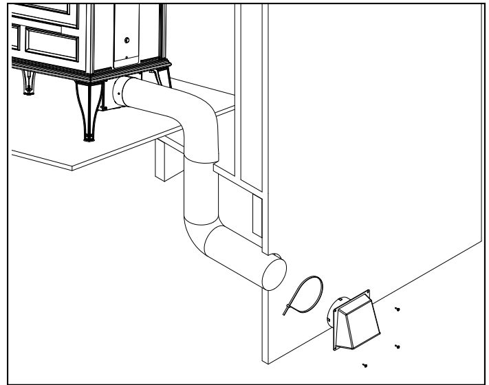
Figure 5.4 - Installation au sol
