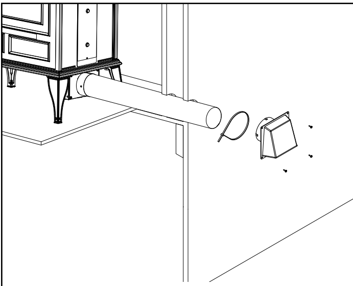
Figure 5.3 - Installation arrière
